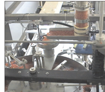
Filler Controls Integrated With Scale
