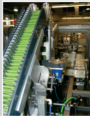
Vertical Collator
