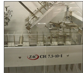
Quick Changeover Carton Pockets
