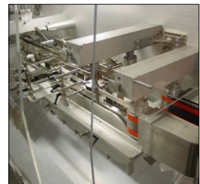
Balcony Style Machine (GMP Design)
