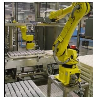
Robotic Loading and Unloading of Pallets
