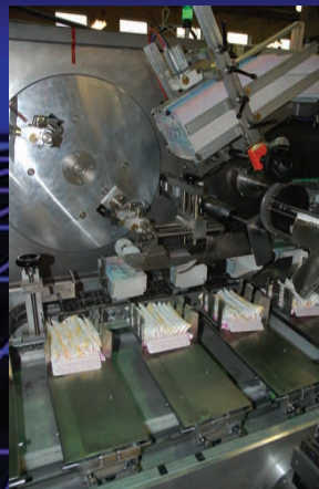
Patented Carry-In Loading Patent 6.912.826
