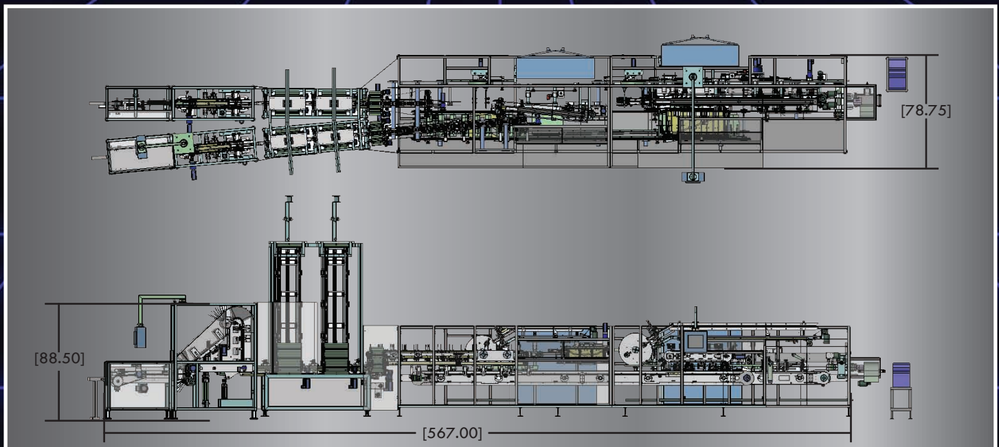
Dual Product Vertical Collation Systems for Variety Pack
