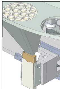
3-D Model of Volumetric Filler Count
