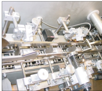
Servo Adjustable Carton Cell Chain
