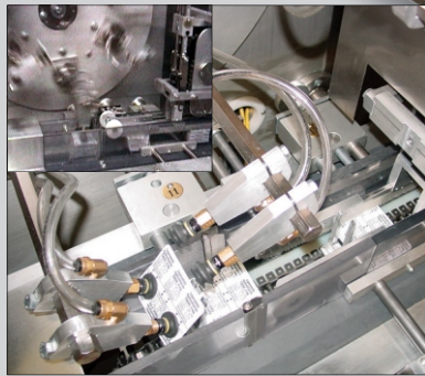
1 to 10 Blister Stacking Capability
